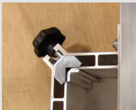
Insert-foot with adjustable load distributor
